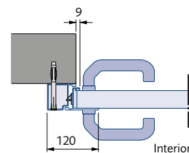
Profile 2: Opening inwards or outwards (inwards shown)
