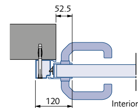
Profile 2: Opening inwards or outwards (inwards shown)
