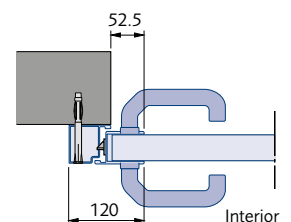
Profile 2: Opening inwards
