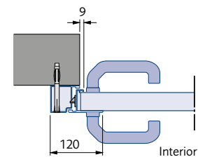
Profile 2: Opening inwards
